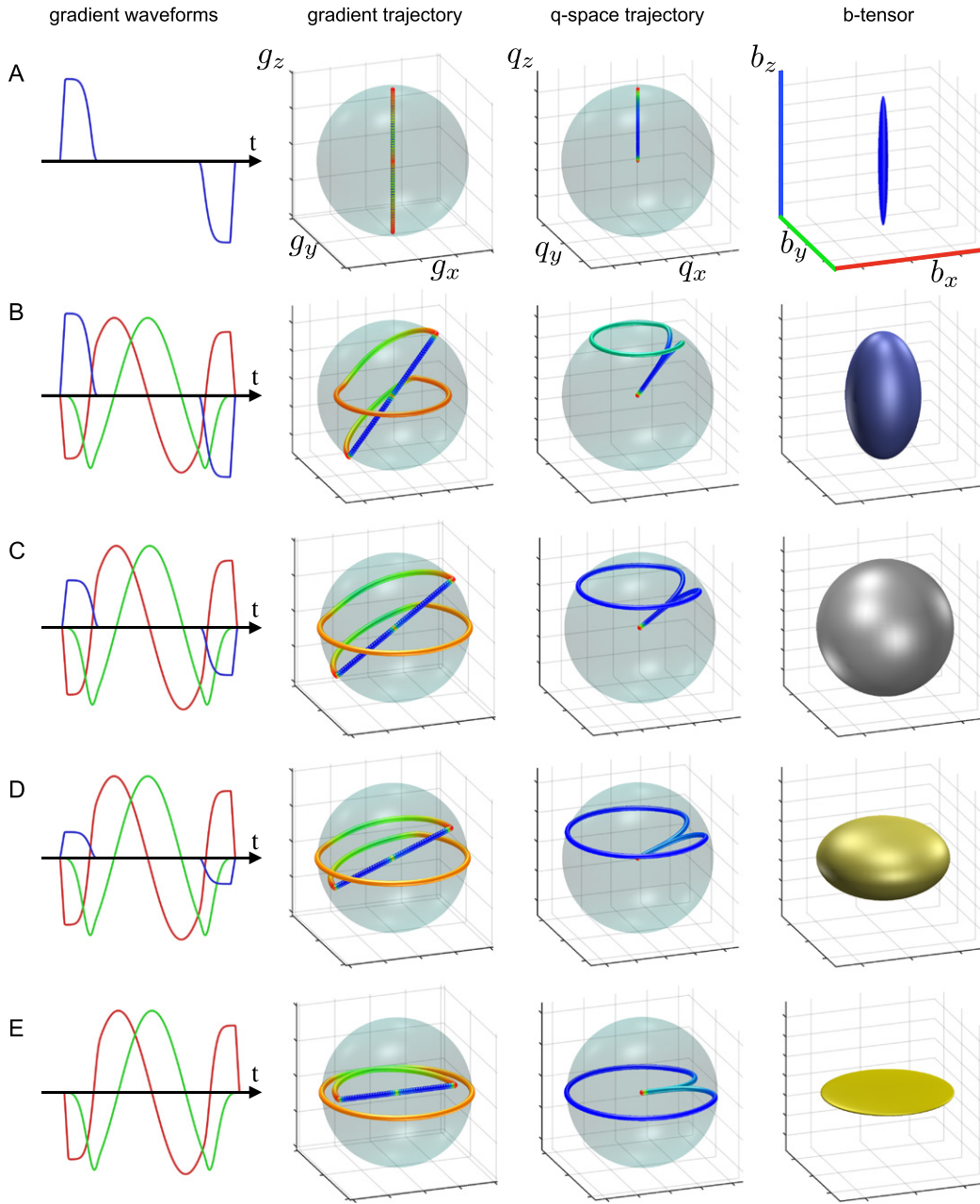
Fig. 4. QTE encoding: an example family of b-tensors, with shapes ranging from linear to spherical to planar. Gradient waveforms and trajectories are shown along with the resulting q-space trajectories and b-tensors. The curves were produced by transforming the curve with efficient isotropic encoding (C) to yield linear encoding (A), prolate encoding (B), oblate encoding (D), and planar encoding (E). We have used b-tensors from this family in our proof-of-concept clinical study, where multiple rotated versions of this family were applied.
