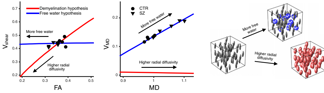
Fig. 12. Comparison of measured data to simulations of two hypothesized pathologies in schizophrenia. Scatter plots show V_{\text{shear}} versus FA (left) and V_{\text{MD}} versus MD. Data points represent an average across the cerebral white matter. The two parameters V_{\text{MD}} and V_{\text{shear}} are related to variances of the distribution, corresponding to changes in size, and changes in orientation/shape respectively. FA and V_{\text{shear}} were weakly correlated. MD and V_{\text{MD}} were strongly correlated. Solid lines show results from analysis of data simulated to represent a demyelination hypothesis, i.e. increasing radial diffusivity (red), and a free-water hypothesis, i.e. replacing WM with isotropic freely diffusing water (blue). Example voxels representing these hypotheses is shown to the right.
