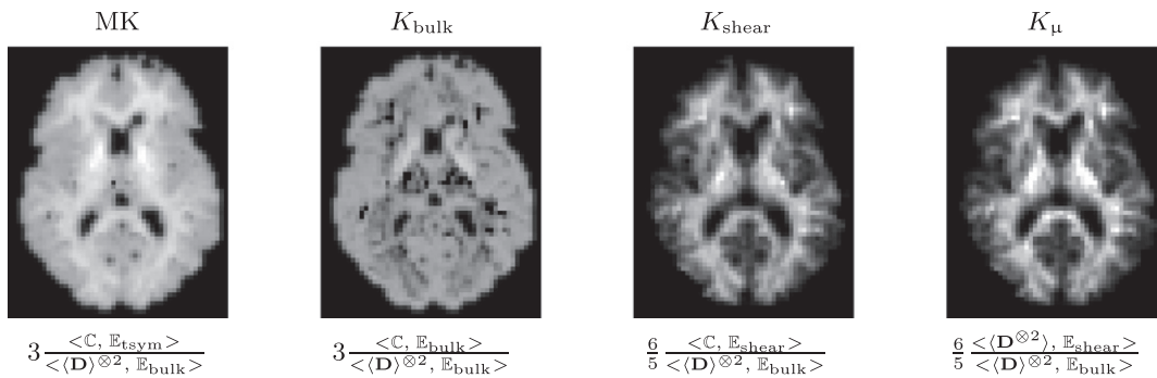
Fig. 9. Examples of parameter maps obtained in QTI, calculated from data acquired with the clinical protocol. A. Top row shows the mean diffusivity MD (Eq. (14)), the bulk V_{MD} and shear variances V_{shear} (Eqs. (19), (22)), and their sum V_{iso} . B. The middle row shows examples of normalized variance measures. C. Lower row shows different kurtosis measures derived from QTI: Total mean kurtosis (MK, Eq. (37)) separated into two components, bulk and mean kurtosis represented by K_{bulk} and K_{shear} (Eqs. (41) and (42)). The anisotropy-related kurtosis K_\mu (Eq. (43)) is shown in the rightmost panel.
