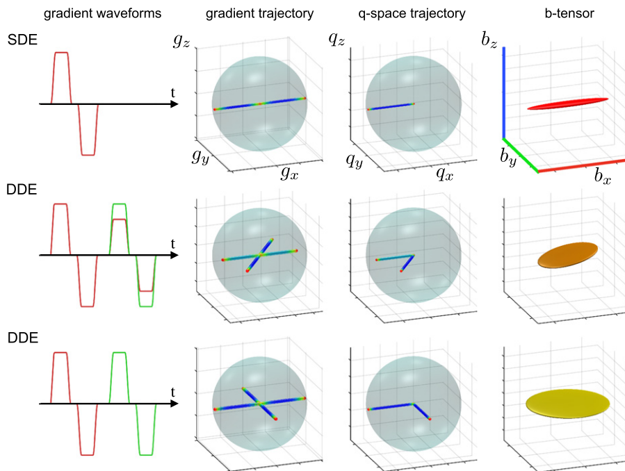
Fig. 2. Examples of gradient waveforms and trajectories that produce “linear” and “planar” b-tensor shapes, from the SDE and DDE experiments. Color coding is as follows: in the gradient waveform column, red–green–blue defines the x–y–z gradient directions; in the gradient trajectory column, slewrate, slow to fast, is encoded by red–yellow–green–blue from zero to max; in the q-space trajectory column, trajectory speed, slow to fast, is encoded red–yellow–green–blue; in the b-tensor column, the diagonal elements of the b-tensor are mapped to red–green–blue. In the rank-1 case, this b-tensor color mapping corresponds to the principal eigenvector direction, analogous to the standard color coding for diffusion tensors. In the planar case, rather than relying on a randomly oriented major eigenvector for color information, the effect is to sum the colors in the plane (as in the bottom row where red plus green gives yellow in the RGB sense).
