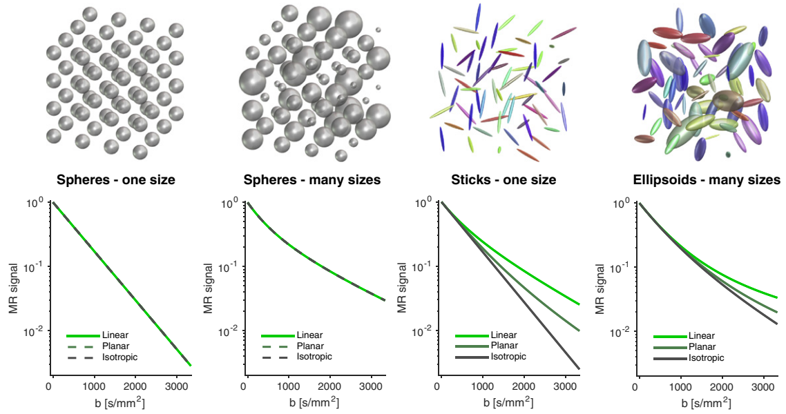
Fig. 6. The signal plots show the MR signal versus b-value measured in four synthetic datasets using b-tensors of three different ranks, where ranks are identified with shapes such that rank 1 is “linear,” rank 2 is “planar,” and rank 3 is “spherical.” The four synthetic datasets represent four distinct scenarios with different distributions of microenvironments (spheres of one size, spheres of many sizes, sticks of one size and multiple orientations, and ellipsoids of multiple sizes and orientations). Notice the similarities of the light green signal curves in the second, third and fourth plots. This illustrates that when using traditional SDE (linear b-tensor), multiple different microenvironments can produce similar signal responses. In fact, they may even be identical. This shows that using simple model-based estimation of the distribution using SDE data and a predefined model of specific shape, a distribution over size and orientation of that shape that fits the data can always be found, but the parameters found will of course be meaningless if the predefined model does not reflect the underlying tissue architecture.
