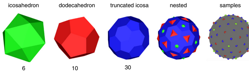
Fig. 7. In the proposed sampling scheme, Platonic solids are used to ensure even sampling in all directions (Westin et al., 2012). The number of distinct sample directions are listed below each solid. Note the dual nature of the icosahedron and dodecahedron: the center of the each face of the icosahedron corresponds to the vertex of the dodecahedron, and vice versa. Further, the center of each face of the truncated icosahedron corresponds to a corner in either the icosahedron or dodecahedron. When the icosahedron, dodecahedron, and truncated icosahedron nest, their vertices (right) give evenly spaced sampling directions. To employ this scheme, a gradient waveform is rotated so that the symmetry axis of its b-tensor aligns with the desired direction (Table 2).
