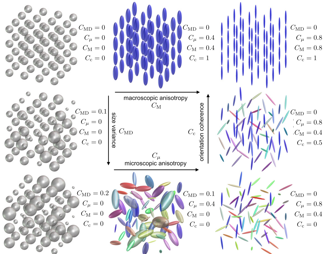
Fig. 5. This visualization of four proposed measures demonstrates how the measures would change in eight illustrative synthetic macrodomains (voxels). Note that these measures intuitively separate size, shape, and orientation coherence, as well as providing the traditional macroscopic anisotropy.
