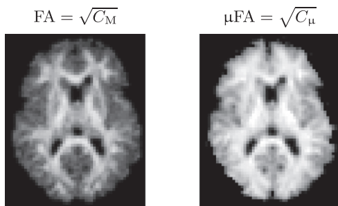
Fig. 10. The anisotropy measure FA and the microscopic anisotropy \mu FA , which is known from previous DDE and qMAS studies (Szczepankiewicz et al., 2015; Lawrenz and Finsterbusch, 2013), are straightforwardly calculated from C_M and C_\mu .
