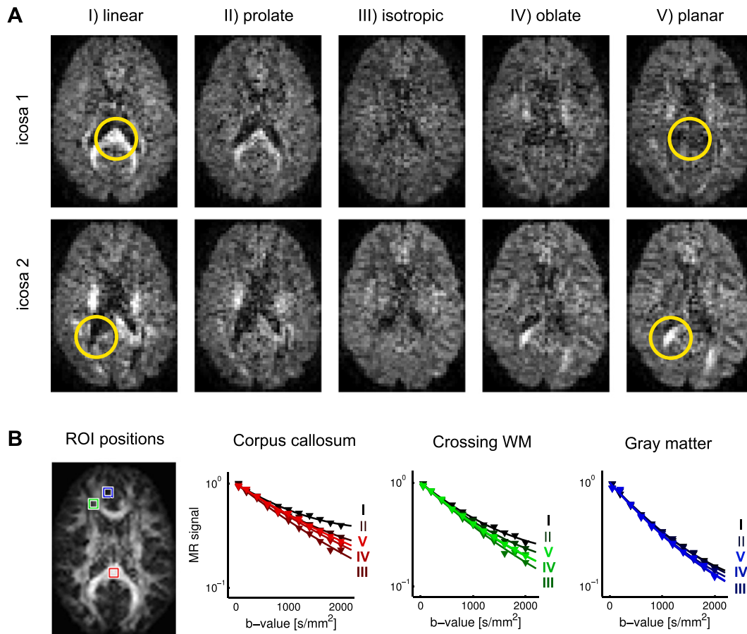
Fig. 8. In vivo data from the preliminary data set. A. MR images diffusion encoded with b = 2000 \text{ s/mm}^2 and b-tensors of five shapes, i.e., linear, prolate, isotropic, oblate, and planar. Data is displayed from two different b-tensor rotations (directions) sampled from the icosahedron (icosa 1 and icosa 2, top and bottom rows). Note that the linear and the planar measurements are dual, and thus, where the linear measurement is bright the planar is dark; see yellow circles. This can be compared to the Funk-Radon transform that is performed in q-ball imaging, where the diffusion signal is the result of integration on a great circle (Tuch, 2004). The planar measurement inherently does this integration. B. Signal-versus-b curves averaged across all directions for corpus callosum (red), crossing white matter (green) and gray matter (blue). Curves are encoded with increasing color brightness from linear (dark, I), through prolate (II), isotropic (III), oblate (IV) to planar encoding (full color, V). As expected, the linear encoding attenuates the signal the least, while the isotropic encoding attenuates it the most, and the attenuations from the other encodings are in between. This in vivo data can be compared to the synthetic curves from Fig. 6, motivating the need for a model, such as the DTD, that can decipher this data.
