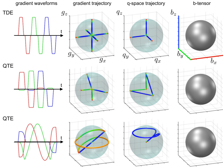
Fig. 3. TDE and QTE encoding schemes can be used to produce isotropic diffusion encoding, with a spherical b-tensor. Color coding is as follows: in column 1, red–green–blue defines the x–y–z gradient directions; in columns 2 and 3, slewrate and trajectory speed are encoded by red–yellow–green–blue, where red is slow and blue is fast; in column 4 the diagonal elements of the b-tensor are mapped to red–green–blue (and thus gray indicates these elements of the isotropic b-tensor are the same). The encoding scheme in the second row was generated by transforming the TDE encoding from the top row: first, pulses were shifted closer together so the green positive pulse aligned with the negative red pulse etc., and then a transform was applied to make the encoding isotropic, as in Eq. (5). In the bottom row, the isotropic diffusion encoding from qMAS produces a lasso-like q-space trajectory.
