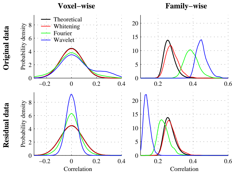
Fig. 2. Theoretical and estimated null-distributions for the correlation coefficient obtained by resampling the synthetic data set. Estimated voxel-wise and family-wise thresholds for a desired p -value can be determined from these distributions, cf. Fig. 1.
