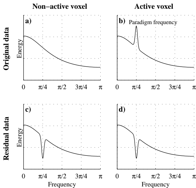
Fig. 4. Schematic spectra of time series in original and residual data (i.e. with a blocked BOLD response model removed from the time series).
