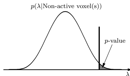
Fig. 1. The null-distribution is the distribution of a test statistic \lambda given that there is no activity in the examined voxel(s). The p -value is the probability of observing a value of the test statistic exceeding the threshold.
